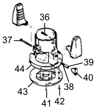
14-4040 Router Base
