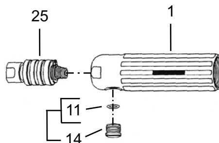
"Q" Push-Pull Throttle
