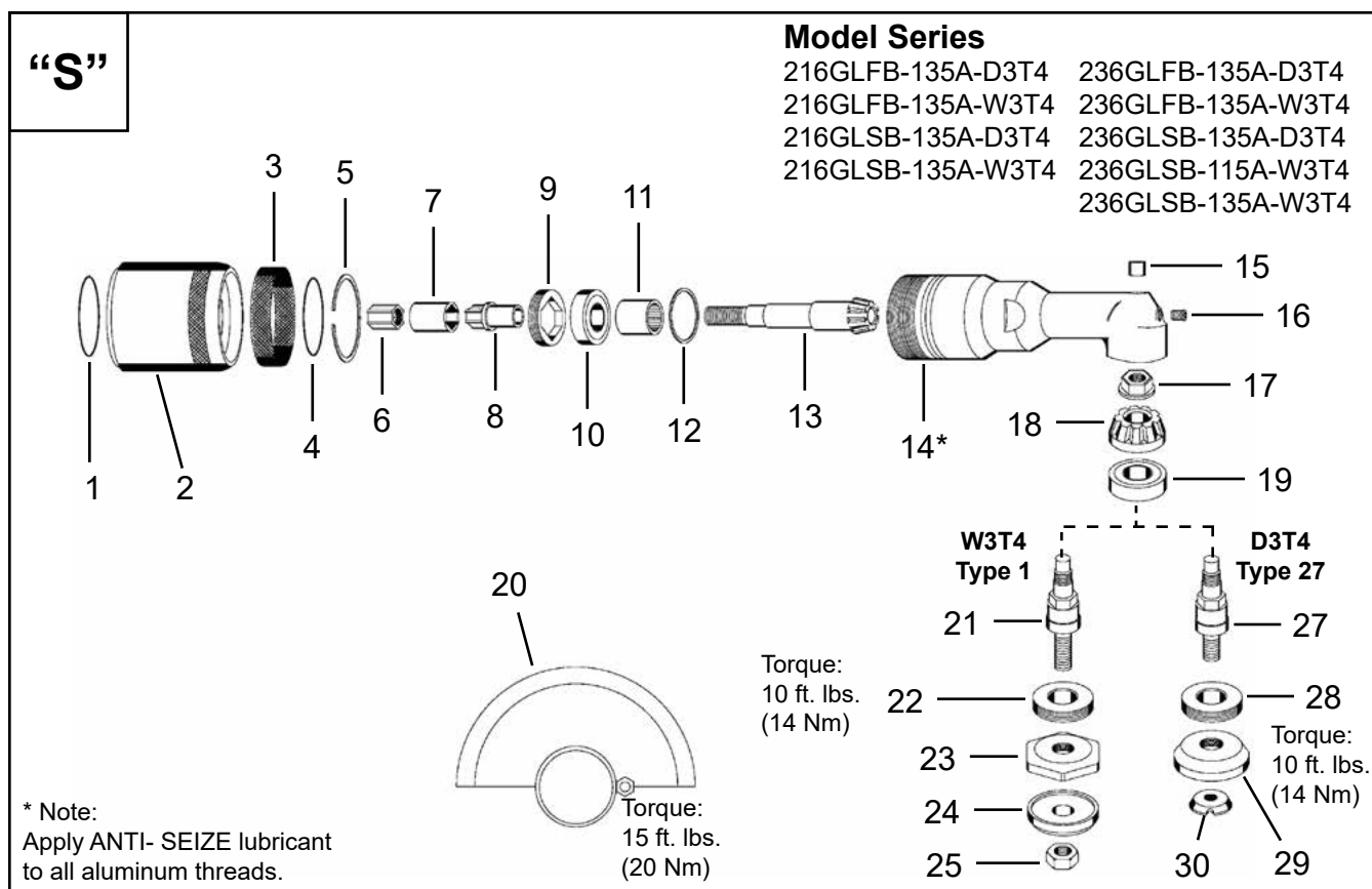
Illustration S: 216G/236G Series Right Angle Front/Side Exhaust Terminations D3T4, W3T4
